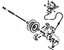
Exploded view of L900
